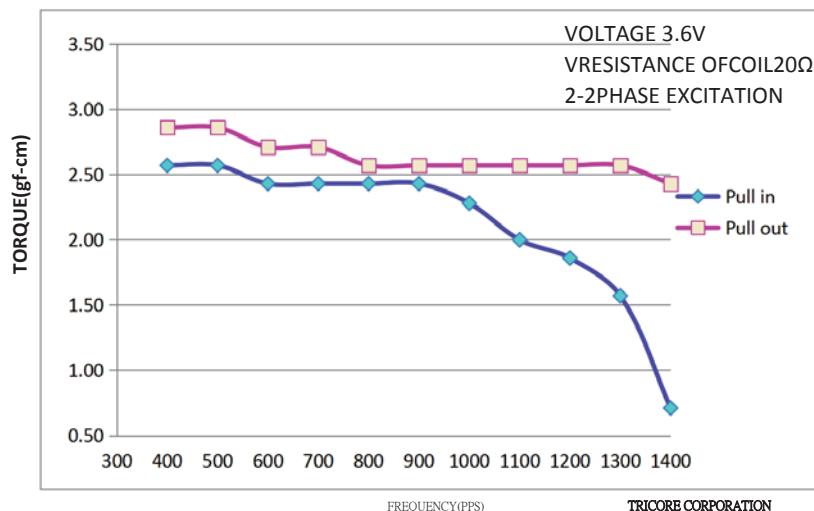
21SRB0607042 STEPPINGMOTOR
