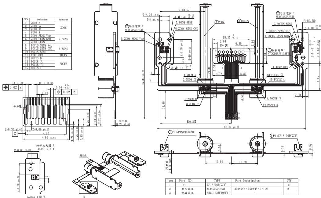
21SRB0607042 STEPPINGMOTOR
